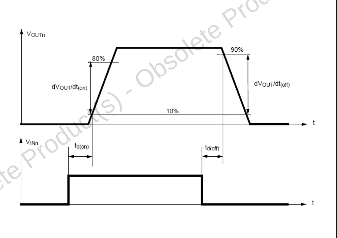
Figure 5. Switching characteristics
