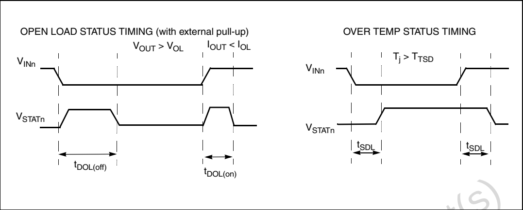
Figure 4. Status timings
