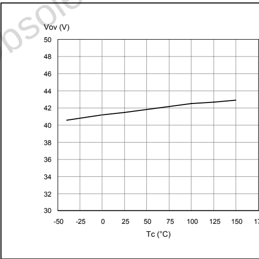
Figure 11. Overvoltage shutdown
