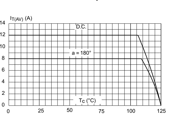
Figure 2. Average and DC on-state current versus case temperature
