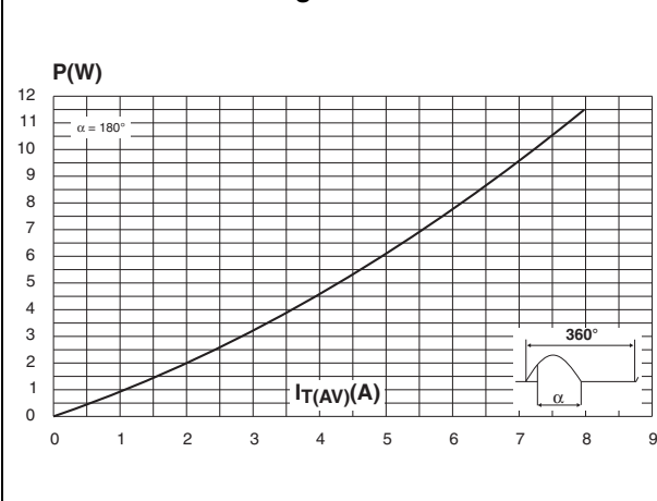
Figure 1. Maximum average power dissipation versus average on-state current
