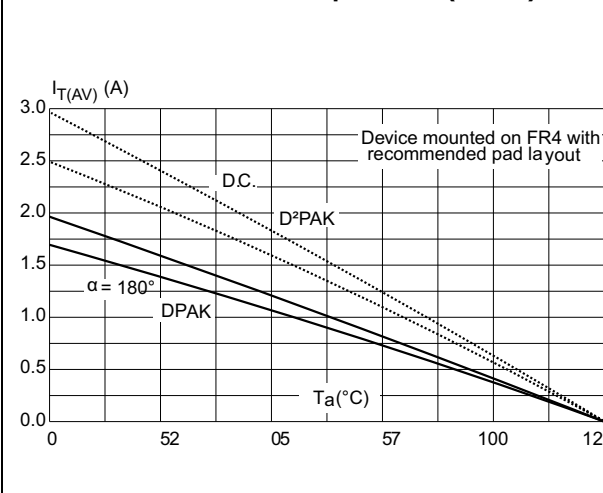
Figure 3. Average and DC on-state current versus ambient temperature (DPAK)
