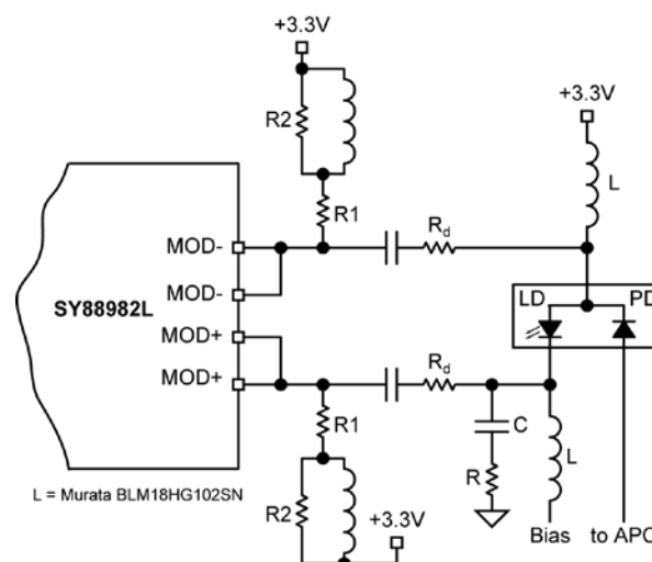
Figure 4. Laser AC-Coupled
