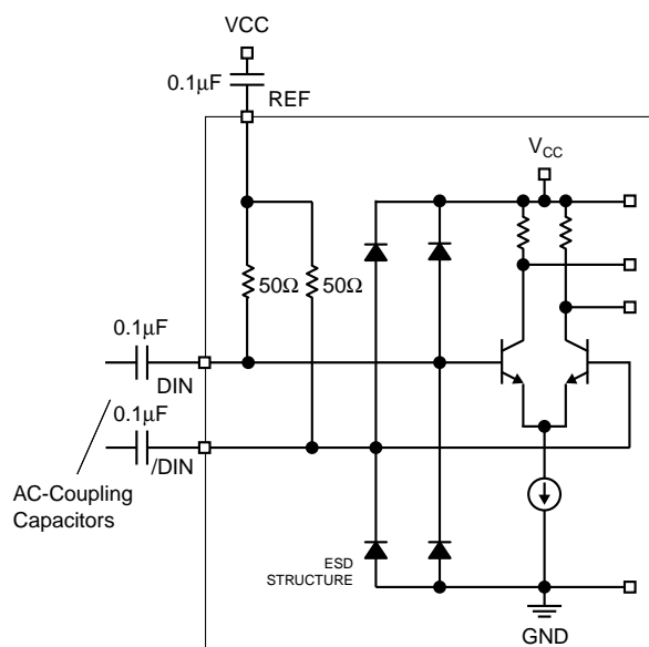
Figure 2. Input Structure
