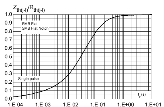
Figure 4. Relative variation of thermal impedance junction to lead versus pulse duration (SMB flat, SMB flat Notch)
