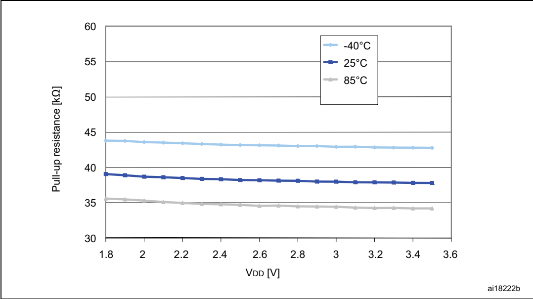
Figure 28. Typical pull-up resistance R_{PU} vs. V_{DD} with V_{IN}=V_{SS}
