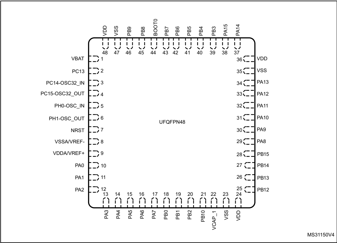
Figure 7. UFQFPN48 pinout
