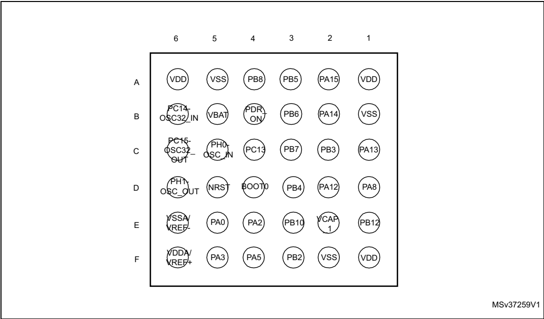
Figure 9. WLCSP36 pinout
