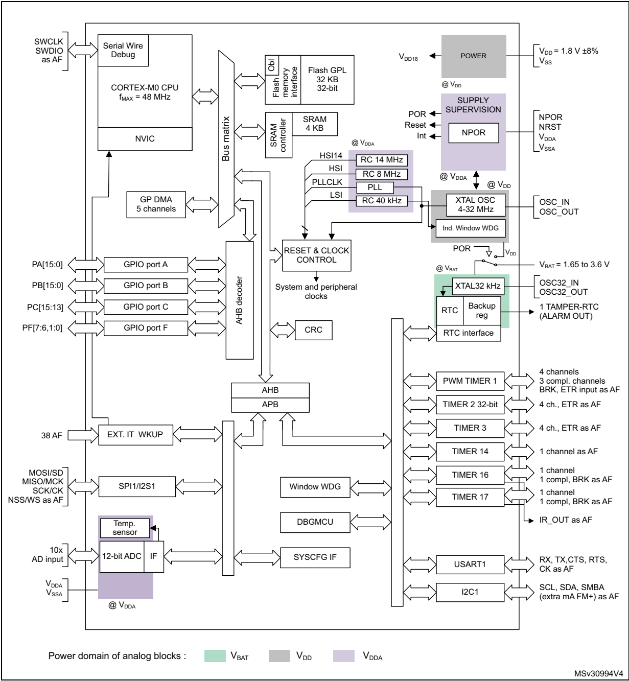
Figure 1. Block diagram
