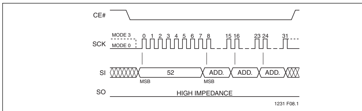
Figure 9: Block-Erase Sequence
