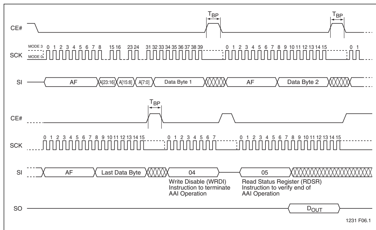
Figure 7: Auto Address Increment (AAI) Program Sequence
