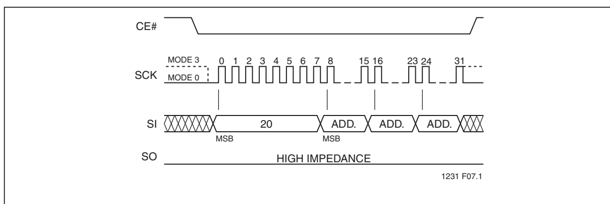
Figure 8: Sector-Erase Sequence
