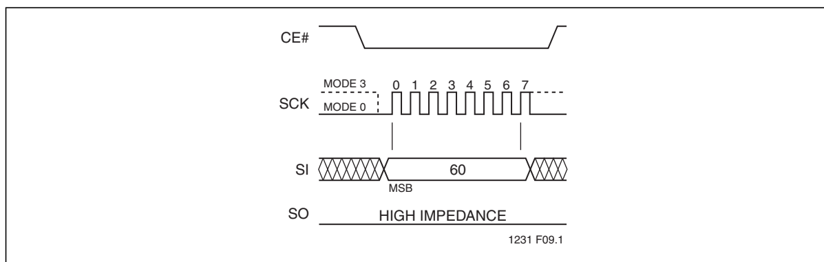
Figure 10: Chip-Erase Sequence
