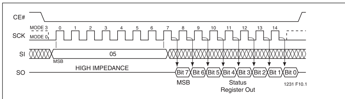
Figure 11: Read-Status-Register (RDSR) Sequence
