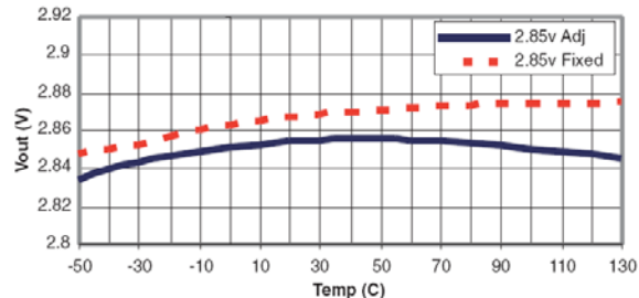
Fig. 12: V_{IN}=4.85V , I_{OUT}=10mA
