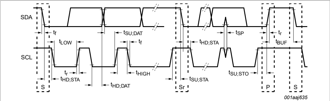
Figure 28. Timing for fast and standard mode devices on the I 2 C-bus
