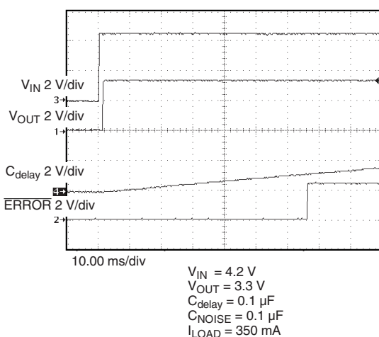
Turn-On Sequence
