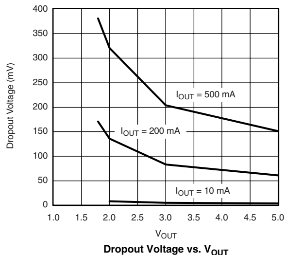
Dropout Characteristic
