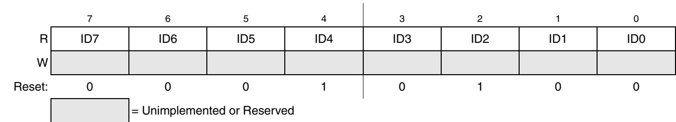
Figure 5-7. System Device Identification Register — Low (SDIDL)
