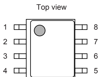
Figure 2 S-35390A-J8T1x
