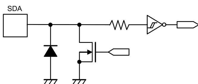
Figure 5 SDA Pin
