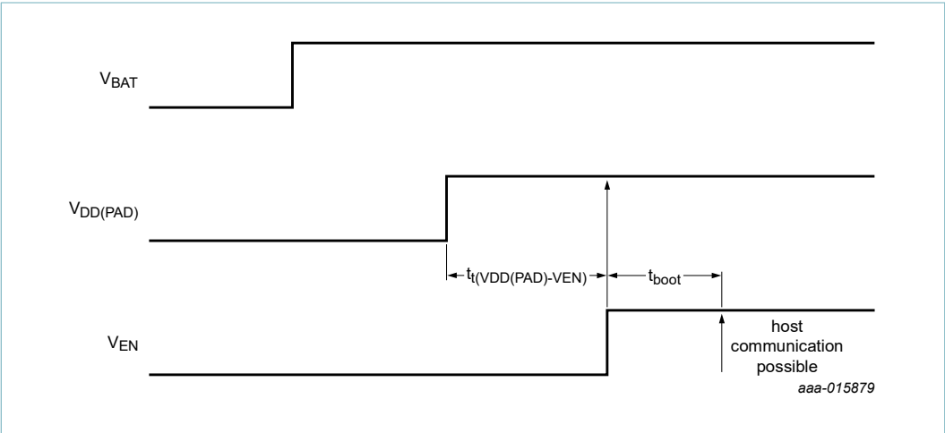
Fig 19. V_{BAT} is set up before V_{DD(PAD)}
