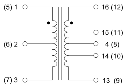
SCHEMATIC "9"
