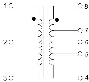
SCHEMATIC "16"
