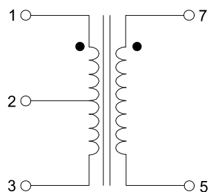
SCHEMATIC "18"
