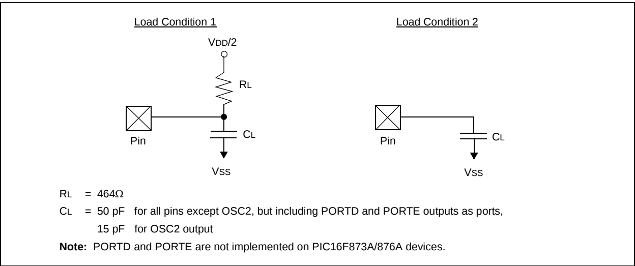
FIGURE 17-3: LOAD CONDITIONS
