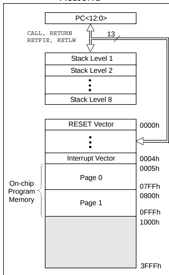
FIGURE 2-2: PROGRAM MEMORY MAP AND STACK OF THE PIC16C771
