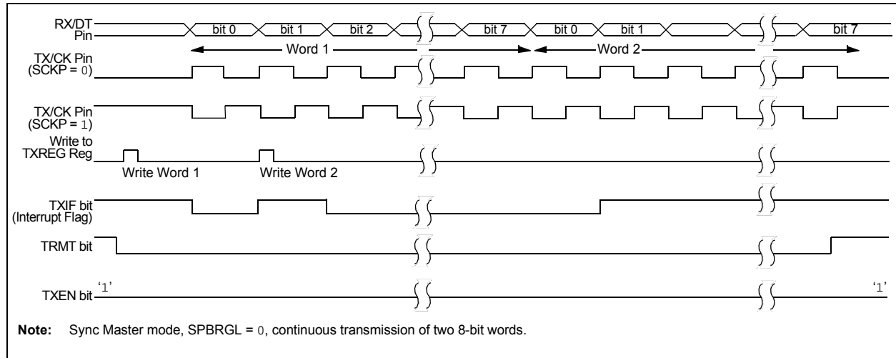
FIGURE 21-10: SYNCHRONOUS TRANSMISSION
