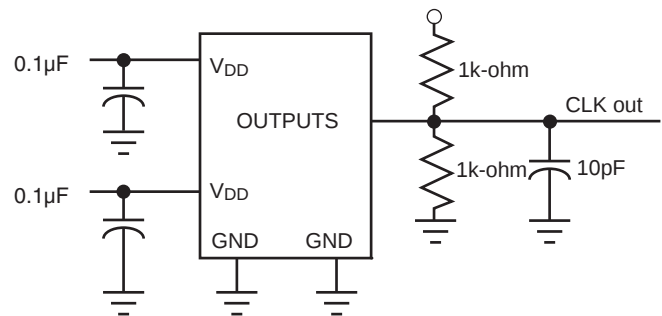
Test Circuit 2
