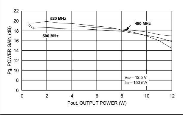
Figure 18. Power gain vs. output power
