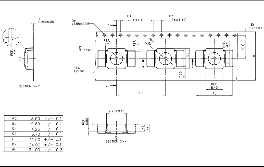
Figure 31. Reel information
