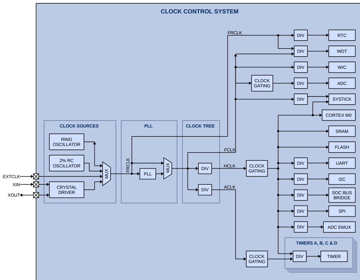
Figure 15-1 Clock Control System
