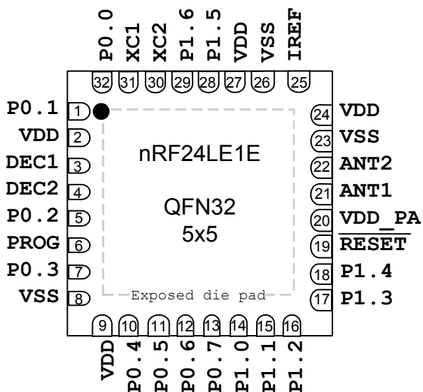
Figure 3. nRF24LE1E pin assignment (top view) for a QFN32 5×5 mm package
