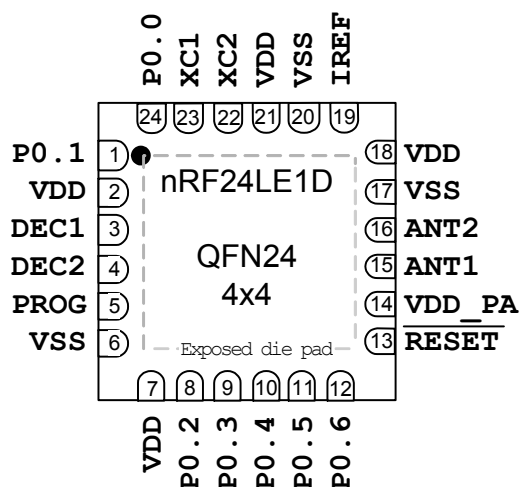
Figure 2. nRF24LE1D pin assignment (top view) for a QFN24 4×4 mm package
