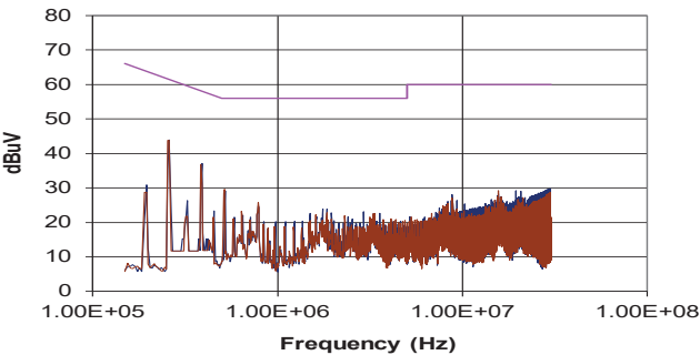
NMK0505TSAC (Quasi-Peak)
