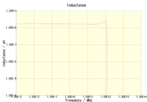
NLCV32T-1R5M-PF
