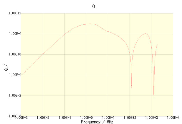
NLCV32T-1R5M-PF
