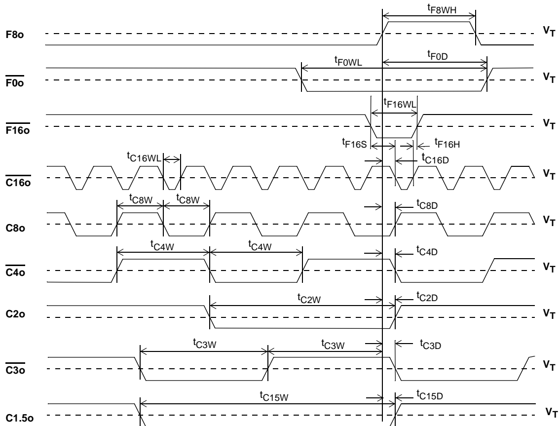
Figure 12 - Output Timing 1
