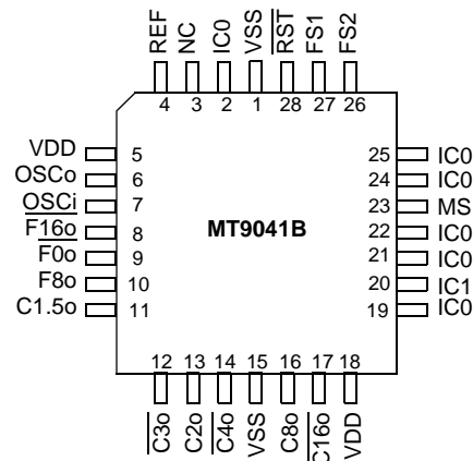
Figure 2 - Pin Connections
