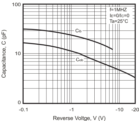
Fig.6 - C_{ob}/C_{ib} — V_{CB}/V_{EB}
