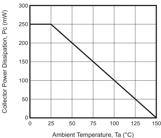
Fig.7 - P_c — T_a
