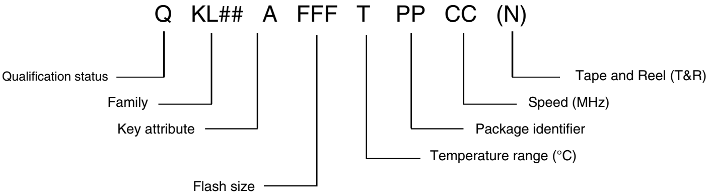
Figure 4. Part numbers diagrams
