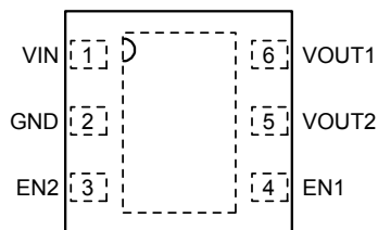
6-pin 1.6mm × 1.6mm Thin MLF® Top View
