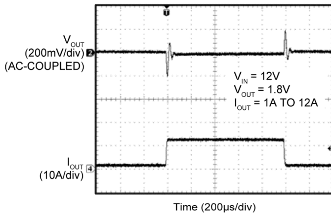
Transient Response
