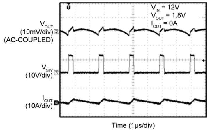
Switching Waveforms
