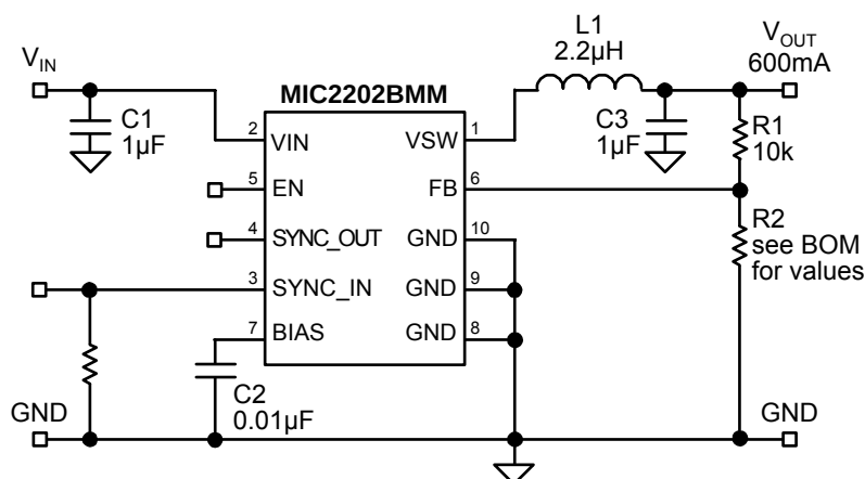
Figure 6. MIC2202BMM Schematic
