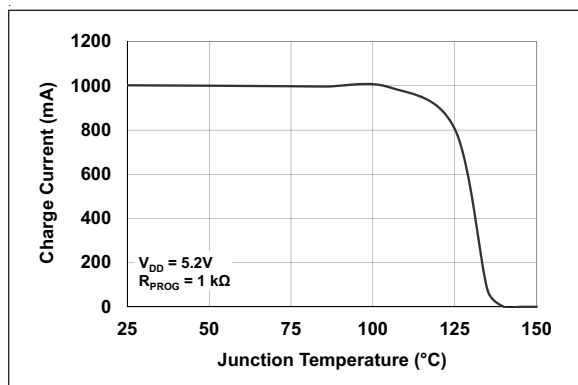
FIGURE 4-3: Thermal Regulation.
