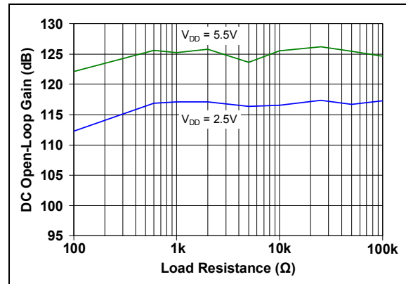
FIGURE 2-11: DC Open-Loop Gain vs. Load Resistance.
