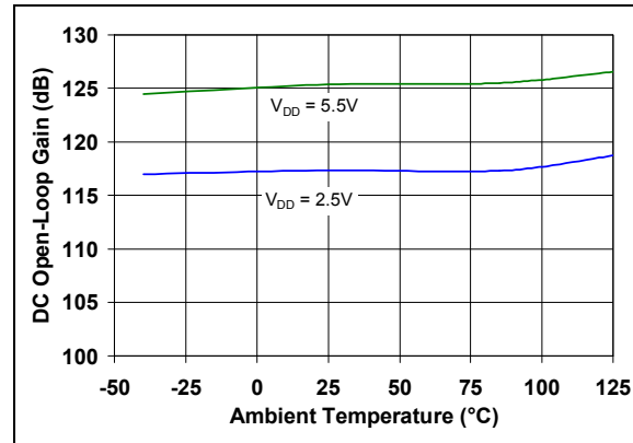
FIGURE 2-10: DC Open-Loop Gain vs. Ambient Temperature.
