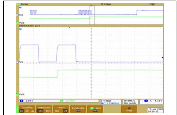
FIGURE 2-20: 5\text{ k}\Omega – Low-Voltage Increment Wiper Settling Time ( V_{DD} = 2.7\text{V} ) ( 1\text{ }\mu\text{s/Div} ).
