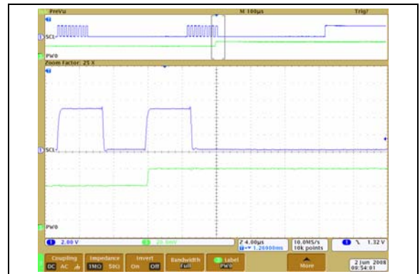
FIGURE 2-21: 5\text{ k}\Omega – Low-Voltage Increment Wiper Settling Time ( V_{DD} = 5.5\text{V} ) ( 1\text{ }\mu\text{s/Div} ).
