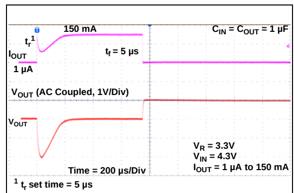
FIGURE 2-59: Dynamic Load Response.
