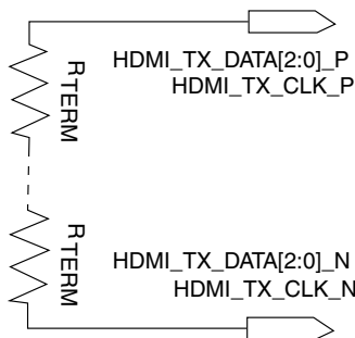
Figure 53. Source Termination
