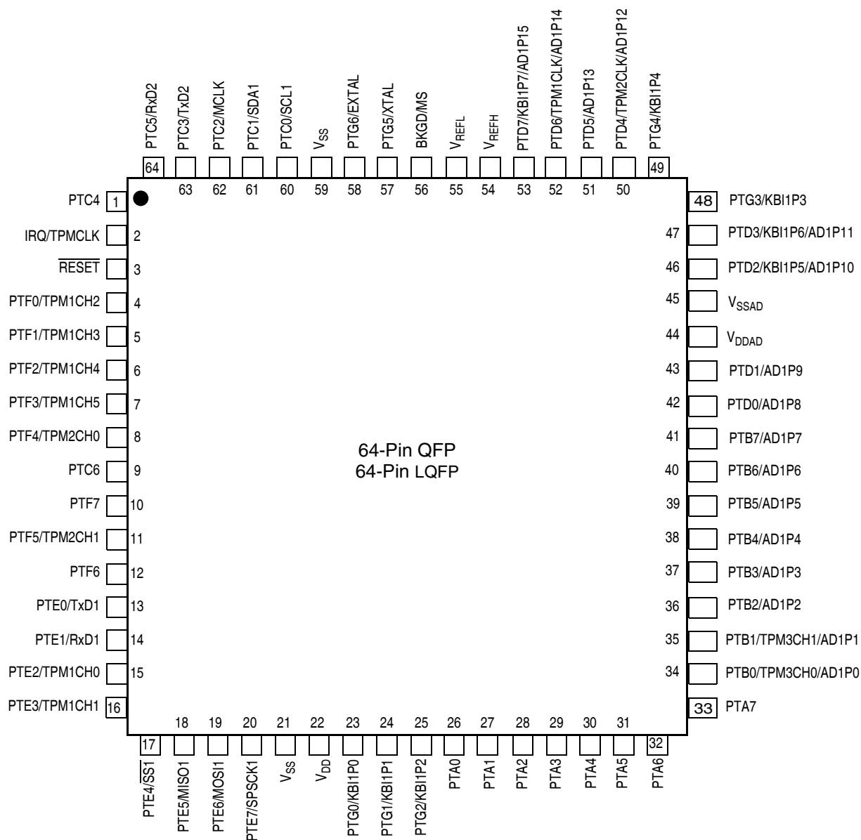
Figure 2-1. MC9S08AC60 Series in 64-Pin QFP or LQFP Package
