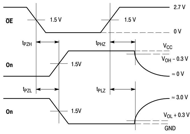
WAVEFORM 2 – OUTPUT ENABLE AND DISABLE TIMES t_R = t_F = 2.5 \text{ ns} , 10% to 90%; f = 1 \text{ MHz} ; t_W = 500 \text{ ns}
