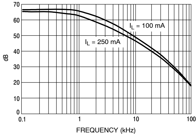
Figure 14. Ripple Rejection
