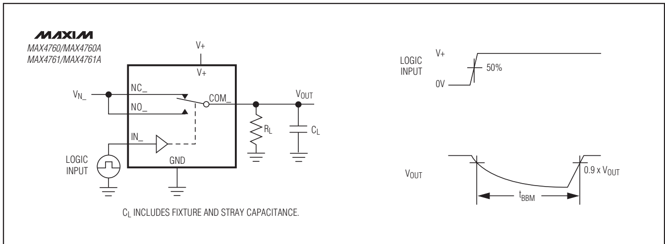
Figure 3. Break-Before-Make Interval
