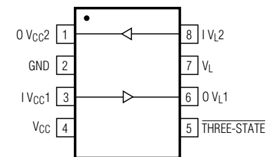
TDFN-8 (3mm x 3mm) TOP VIEW
