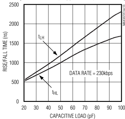
RISE/FALL TIME vs. CAPACITIVE LOAD (DRIVING I/O V_{\text{CC}} , V_{\text{CC}} = +3.3\text{V} , V_L = +1.8\text{V} )
