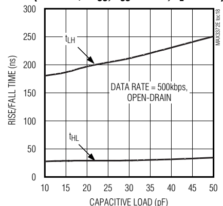
RISE/FALL TIME vs. CAPACITIVE LOAD (DRIVING I/O V_{\text{CC}} , V_{\text{CC}} = +3.3\text{V} , V_L = +1.8\text{V} )
