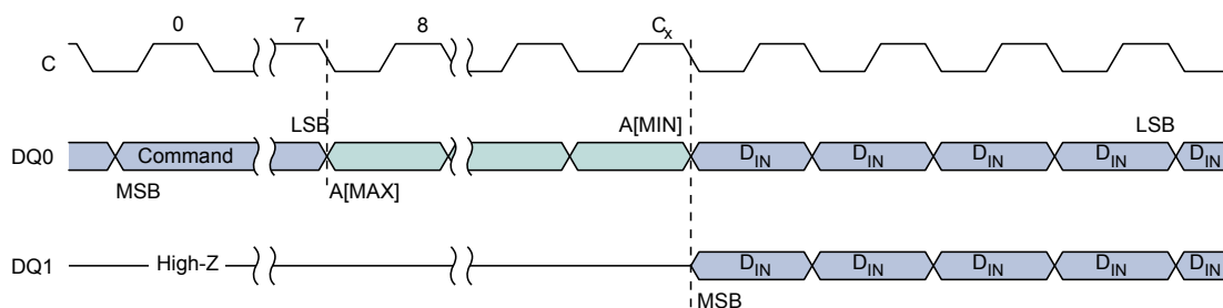
Figure 21: DUAL INPUT FAST PROGRAM Command Sequence
