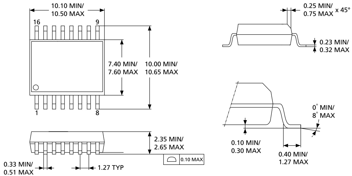
Figure 39: SO16W 300 mils Body Width
