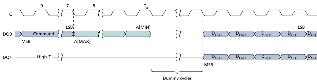
Figure 17: DUAL OUTPUT FAST READ Command Sequence
