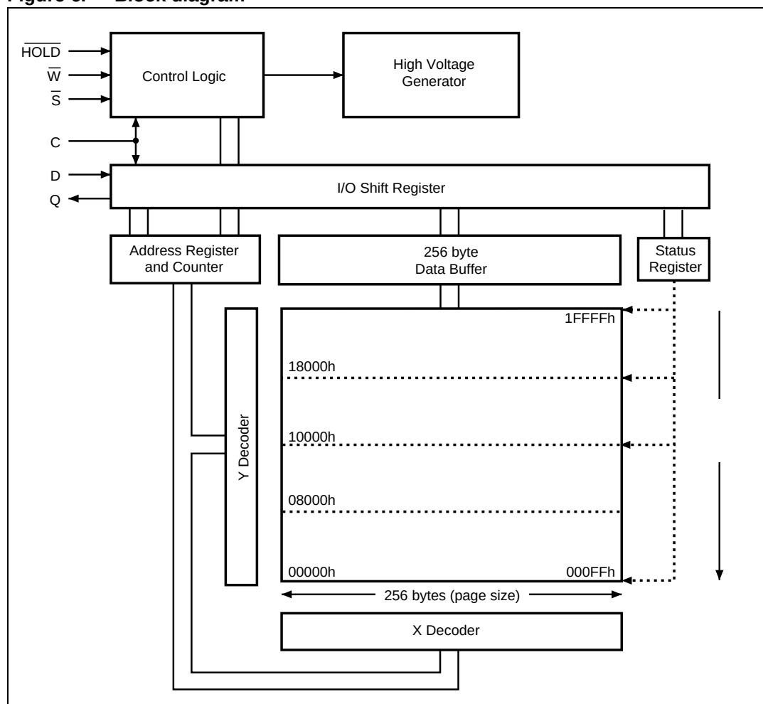
Figure 6. Block diagram
