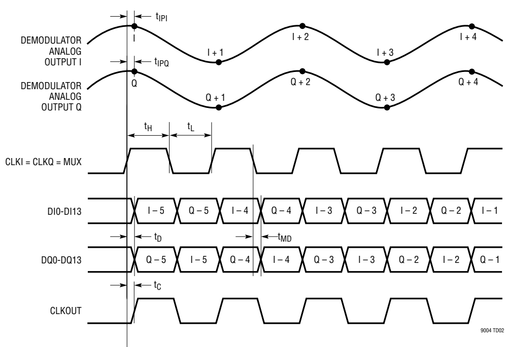
Multiplexed Digital Output Bus Timing
