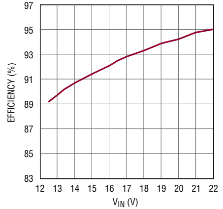
Efficiency vs V_{IN} , Boost Operation, 23.4V at 1A LED String
