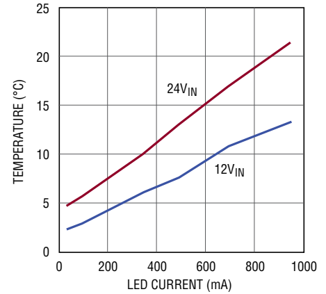
Junction Temperature Rise vs Load, Buck Mode, 8.3V at 1A LED String
