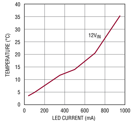
Junction Temperature Rise vs Load, Buck-Boost Mode, 8.3V at 1A LED String
