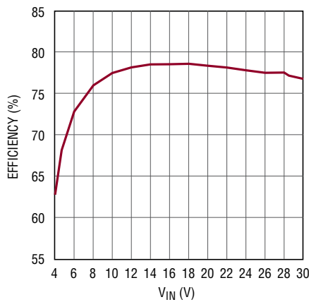
Efficiency vs V_{IN} , Buck-Boost Mode, 3.6V at 1A LED String
