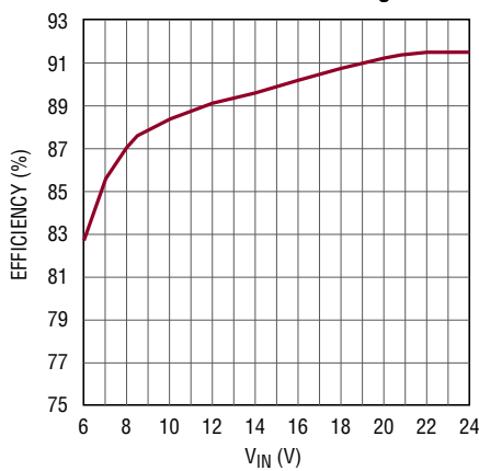
Efficiency vs V_{IN} , Boost Operation, 24.8V at 350mA LED String
