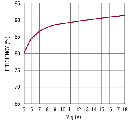
Efficiency vs V_{IN} , Boost Operation, 21.6V at 350mA LED String
