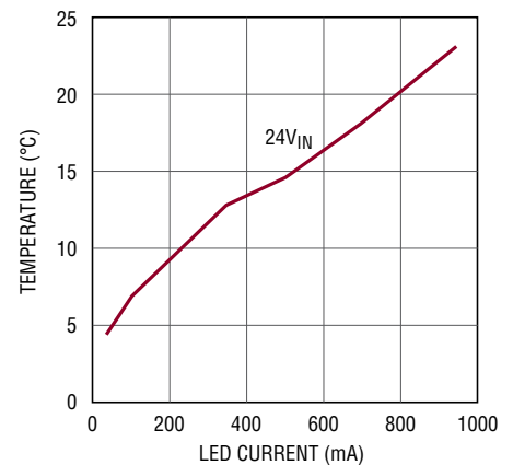
Junction Temperature Rise vs Load, Buck Mode, 18.1V at 1A LED String
