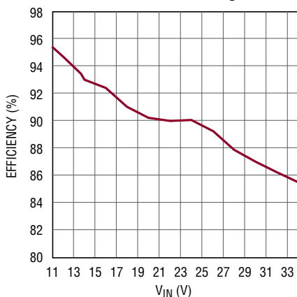
Efficiency vs V_{IN} , Buck Mode, 9.7V at 350mA LED String
