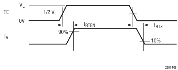
Figure 8. Termination Resistance and Timing Measurements
