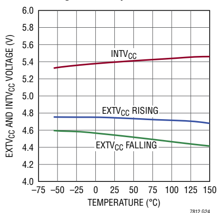
EXT CC Switchover and INTV CC Voltages vs Temperature
