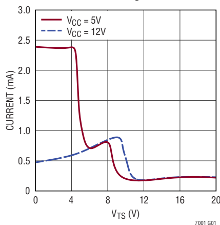
Total Supply Current with External FET ON vs V_{TS} Voltage
