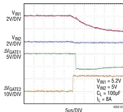
Fast Gate Switchover From Failing Supply
